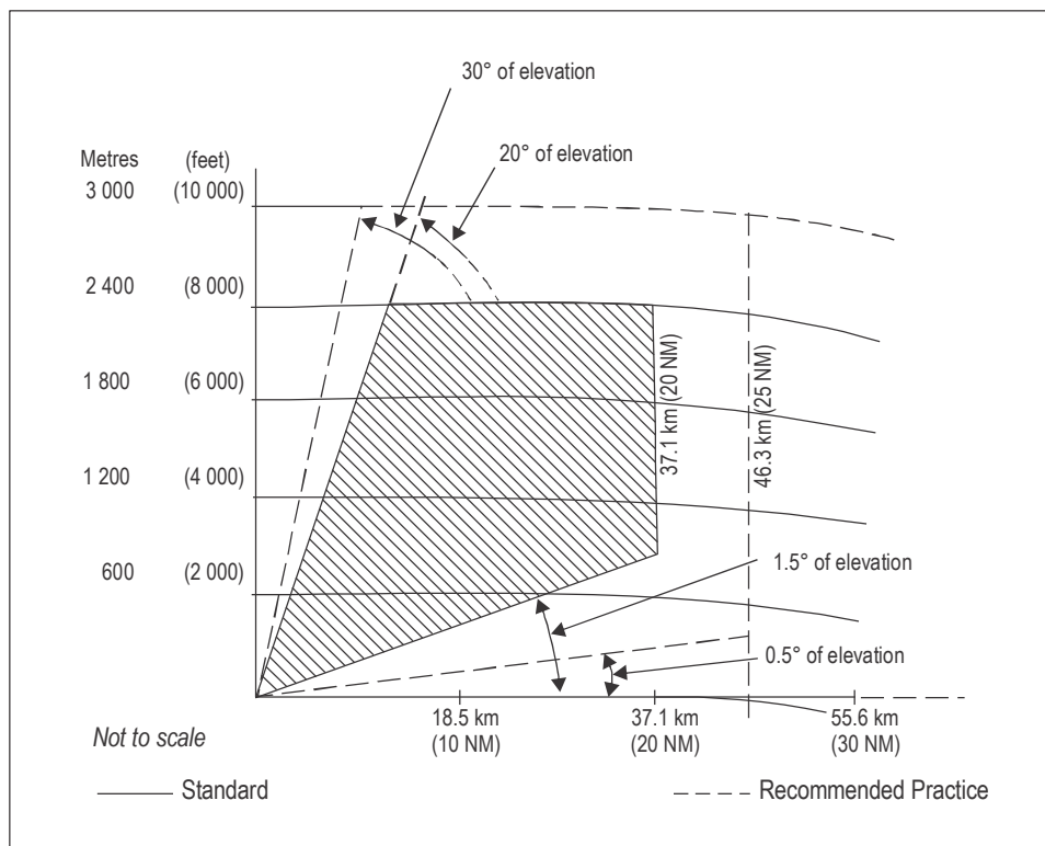
Figure C-18. SRE of precision approach radar system — vertical coverage on a 15 m² echoing area aircraft
