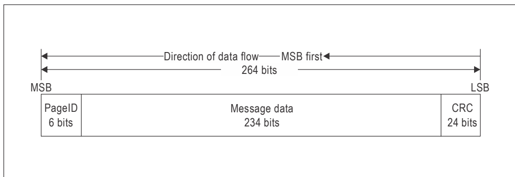
Figure B-22. Frame structure for B-CNAV1 subframe 3
