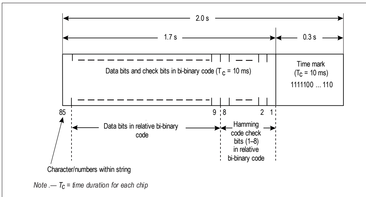
Figure B-10. Data string structure
