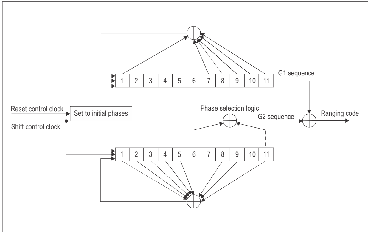
Figure B-19. Generator of CB11
