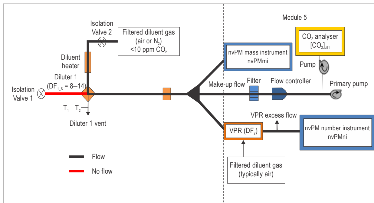
Figure A7-4. Flow schematic for the transfer part cleanliness check
