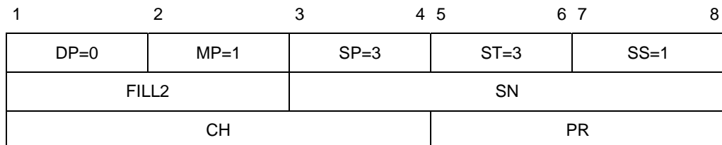
Figure 5-14. REJECT packet
