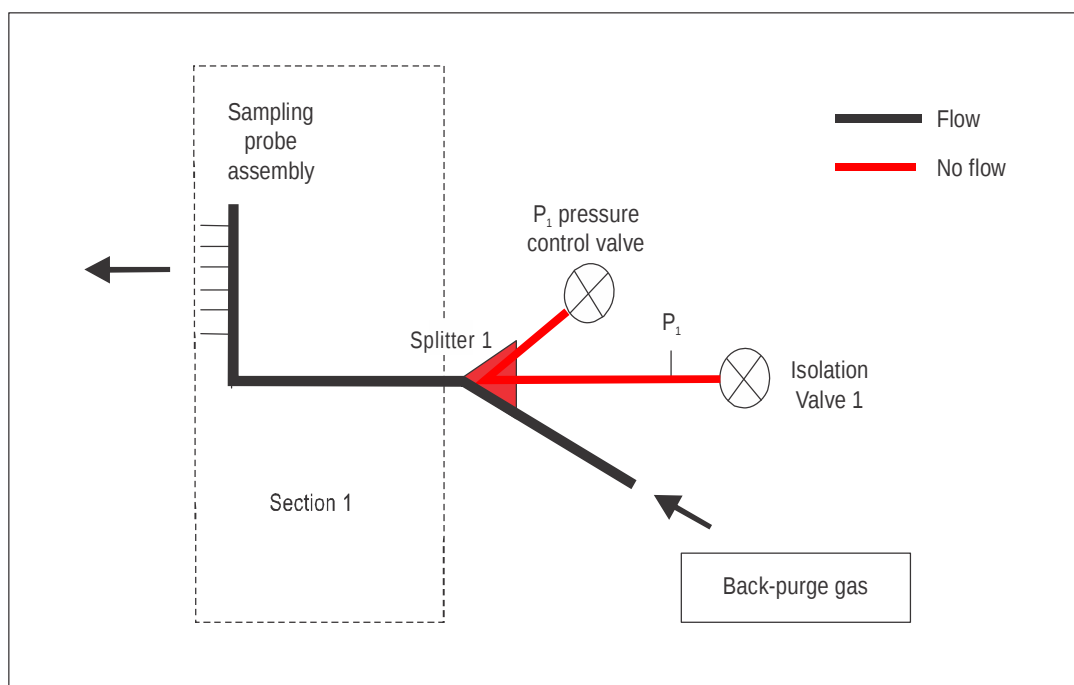
Figure A7-5. Flow schematic for Section 1 back-purge
