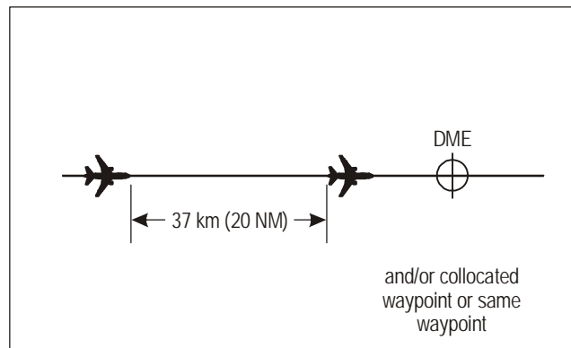
Figure 5-22. 37 km (20 NM) DME and/or GNSS-based separation between aircraft on same track and same level (see 5.4.2.3.1 a))
