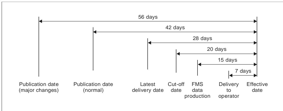
Figure 2-2. Processing cycle for airborne navigation databases
